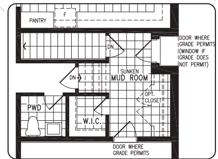
OPTIONAL MUD ROOM ELEVATION B
