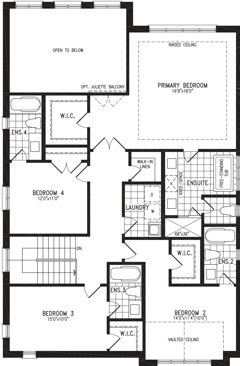
SECOND FLOOR ELEVATION A OPT. LAUNDRY
