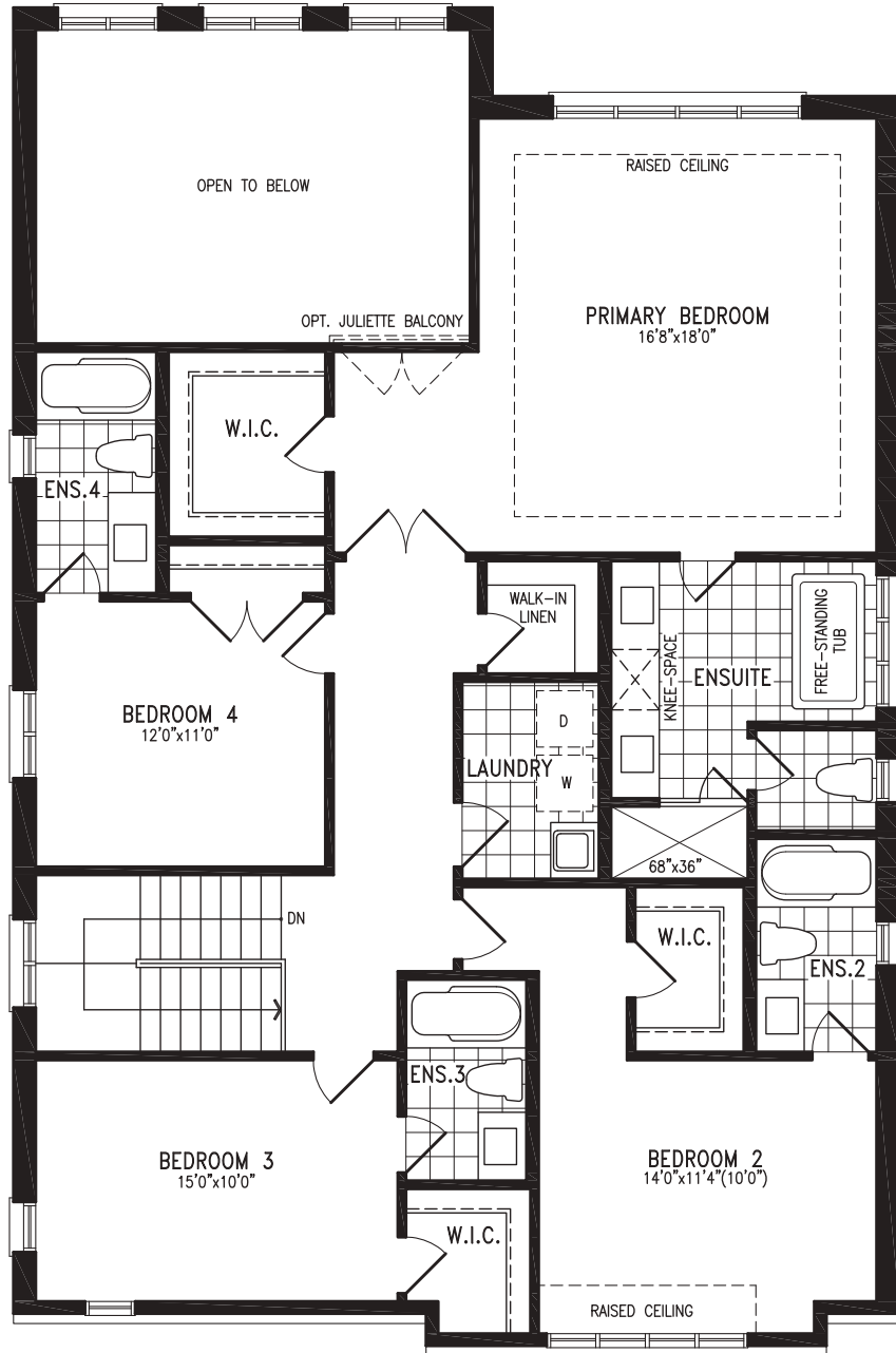
SECOND FLOOR ELEVATION B OPT. LAUNDRY
