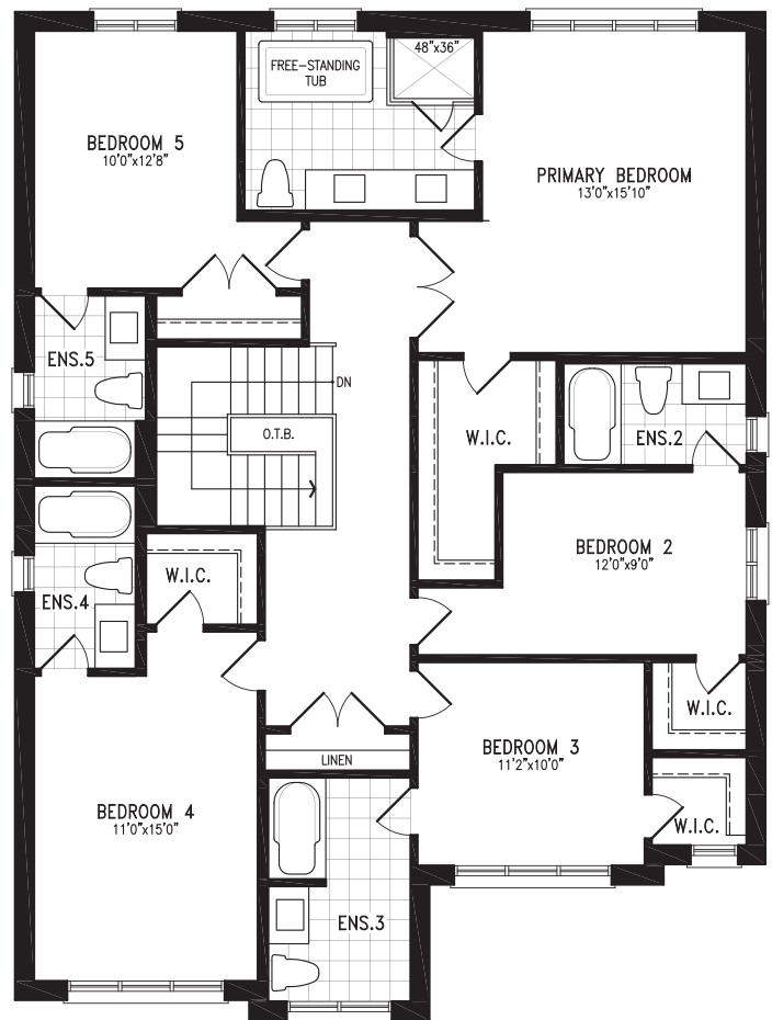
ELEVATION B SECOND FLOOR (OPT. 5 BED)
