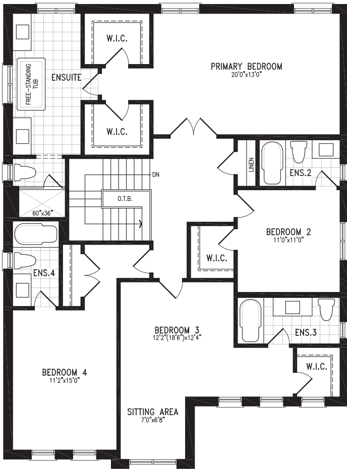
ELEVATION C SECOND FLOOR (STD. 4 BED)
