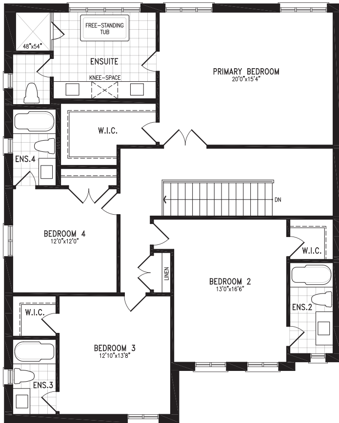
ELEVATION B SECOND FLOOR (STD. 4 BED)
