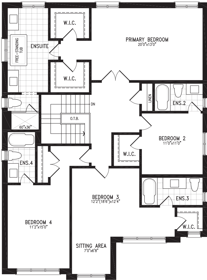
ELEVATION B SECOND FLOOR (STD. 4 BED)
