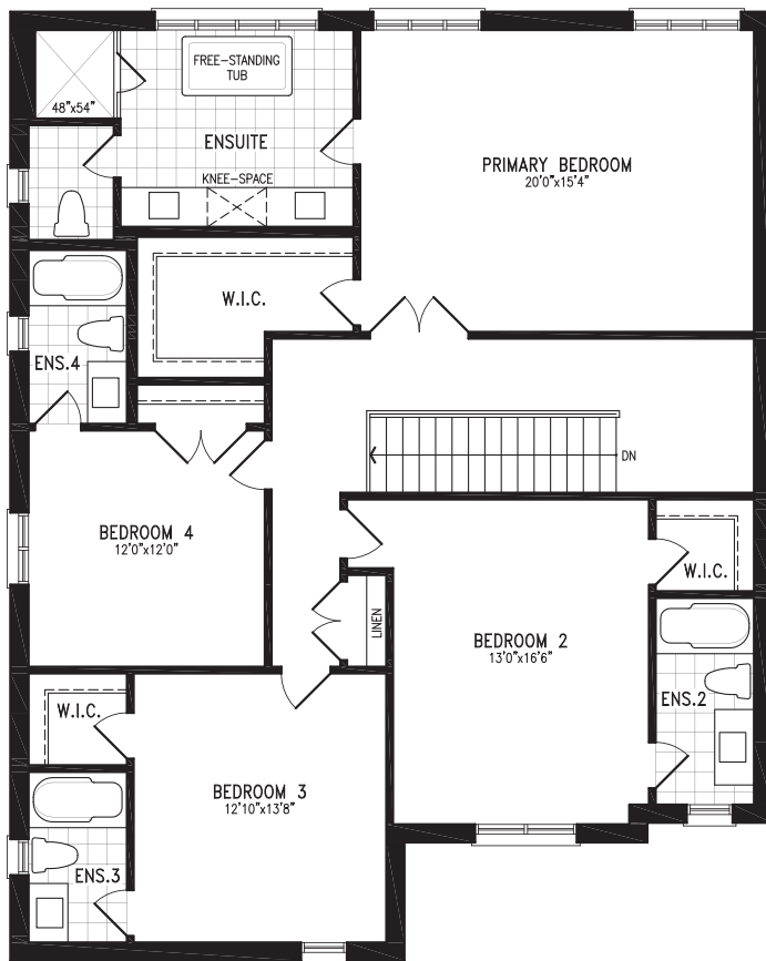
ELEVATION A SECOND FLOOR (STD. 4 BED)
