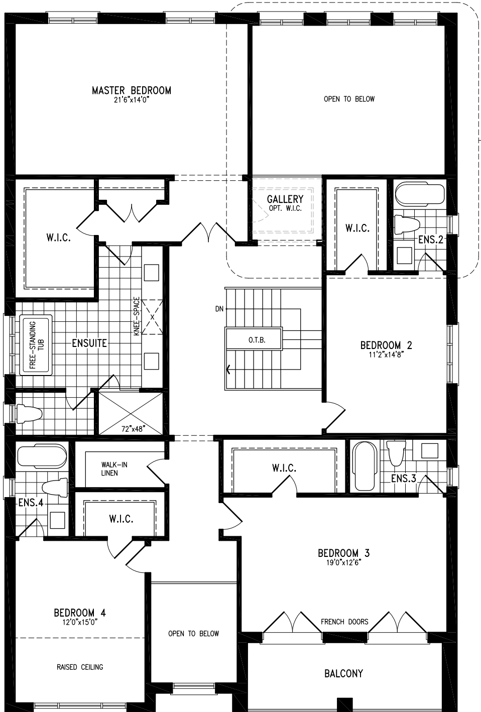
ELEVATION C SECOND FLOOR
