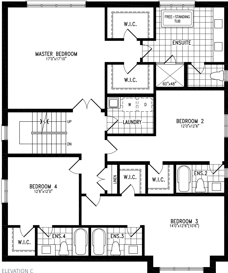
ELEVATION C SECOND FLOOR
