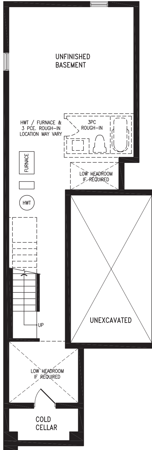
ELEVATION A BASEMENT
