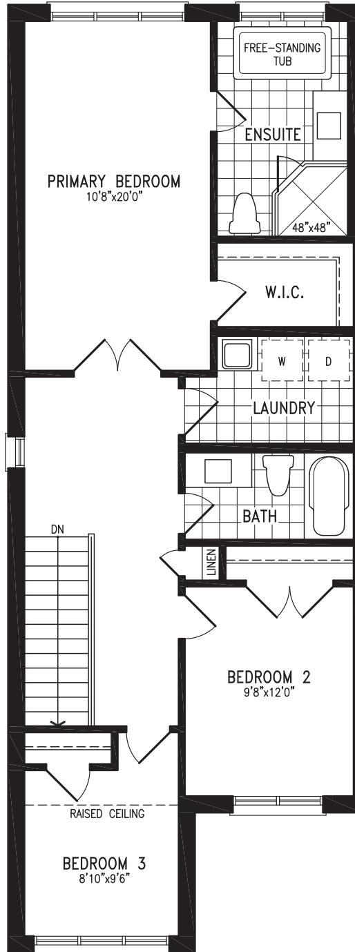
ELEVATION B SECOND FLOOR
