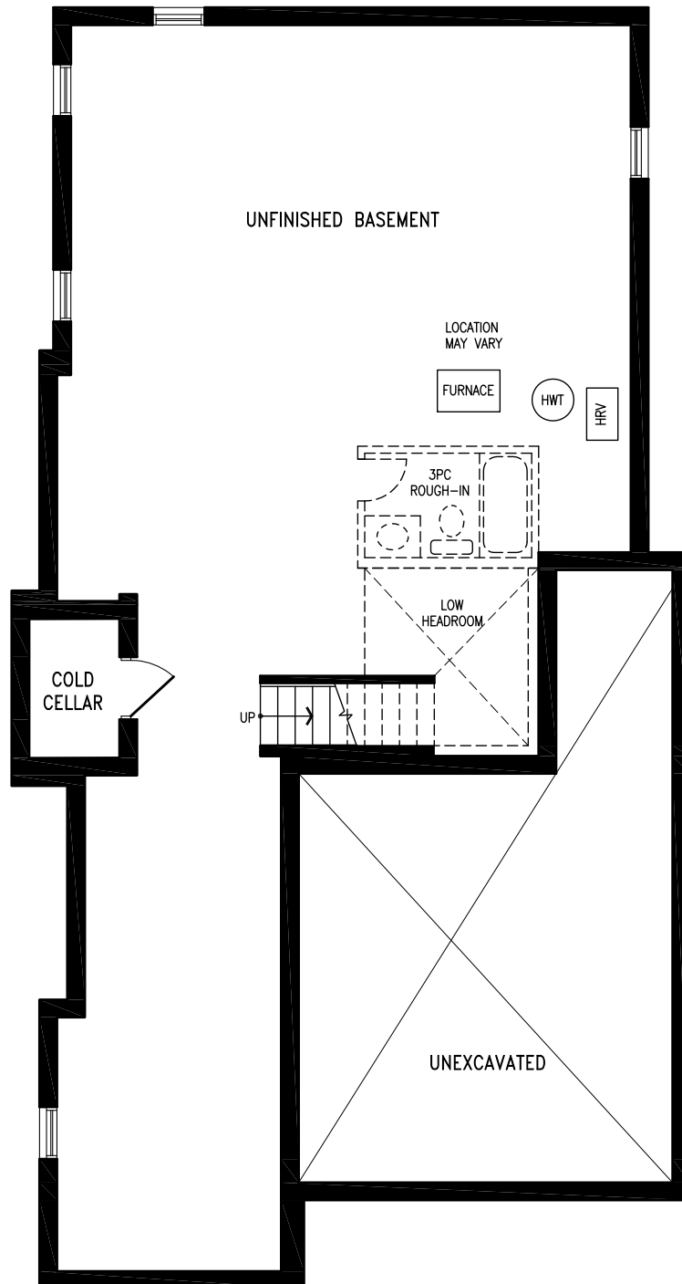
Elevation C BASEMENT
