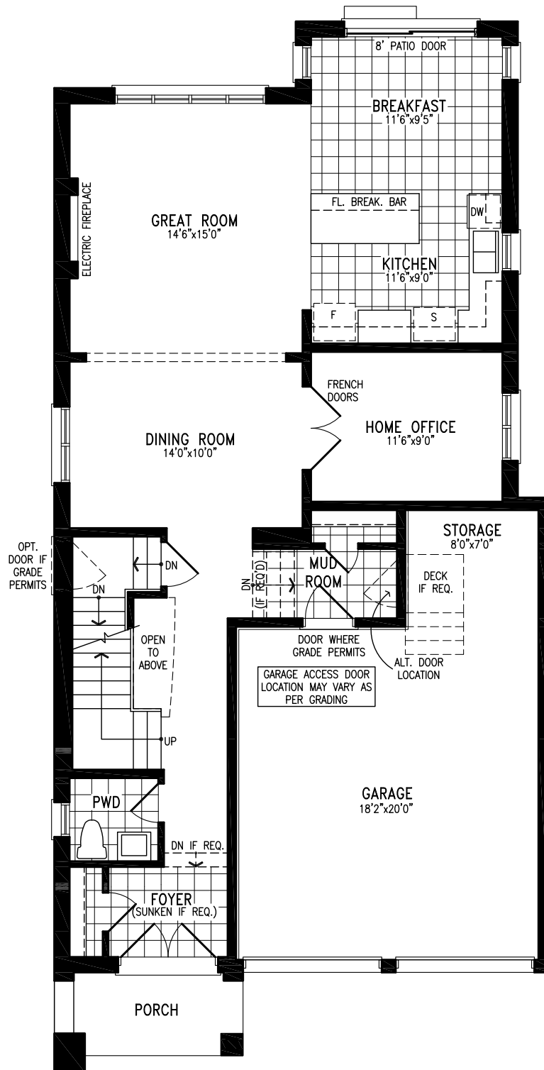
Elevation C GROUND FLOOR
