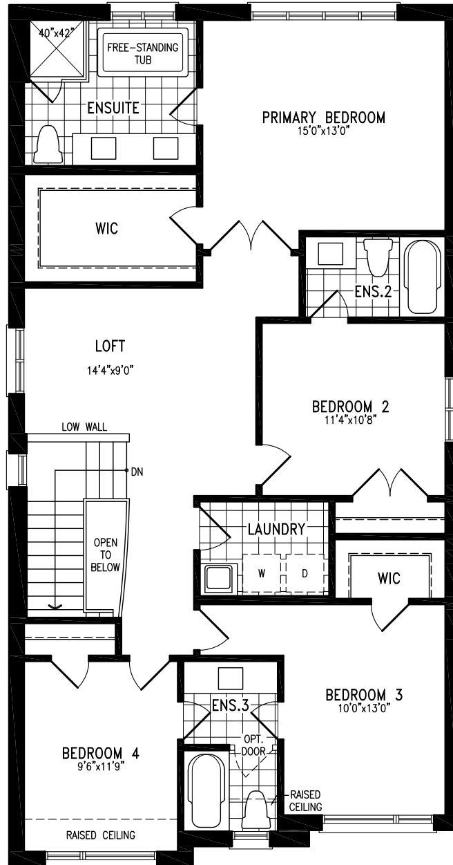
Elevation C SECOND FLOOR
