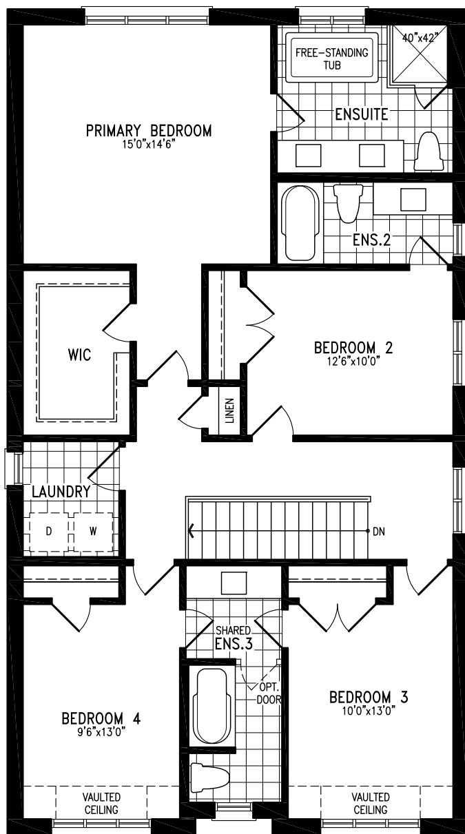
Elevation B SECOND FLOOR
