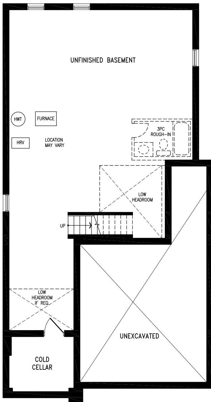
Elevation C BASEMENT
