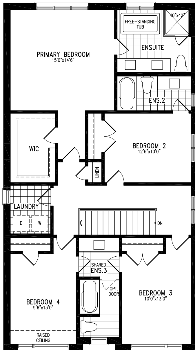
Elevation C SECOND FLOOR
