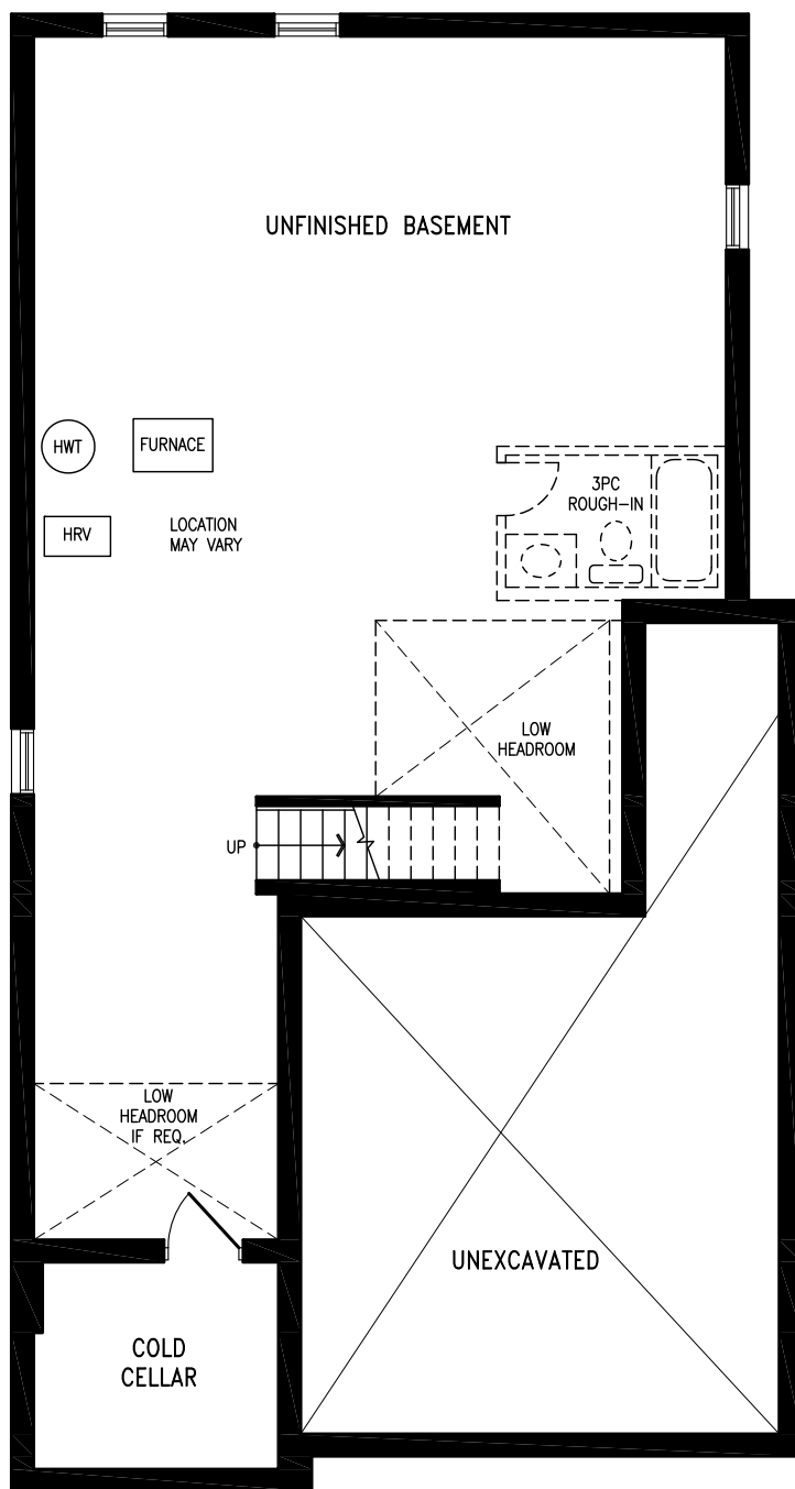
Elevation B BASEMENT
