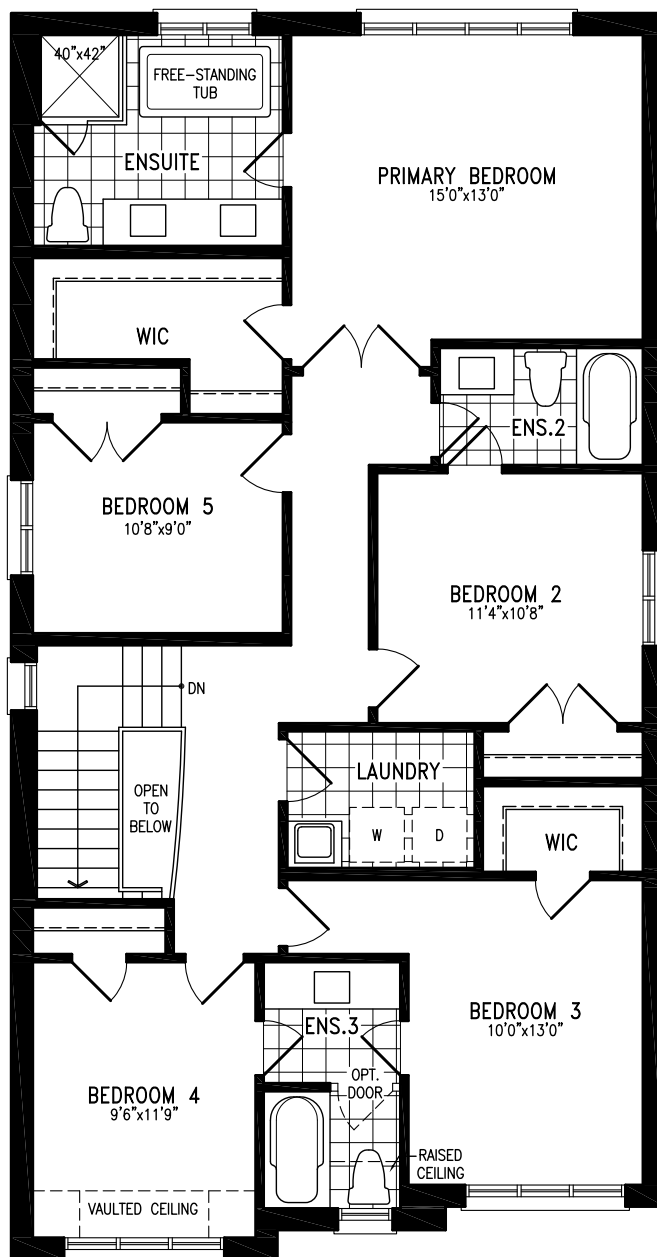
Elevation B OPT. 5 BEDROOM SECOND FLOOR
