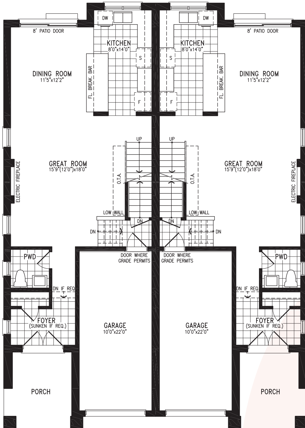
Elevation C1 GROUND FLOOR
