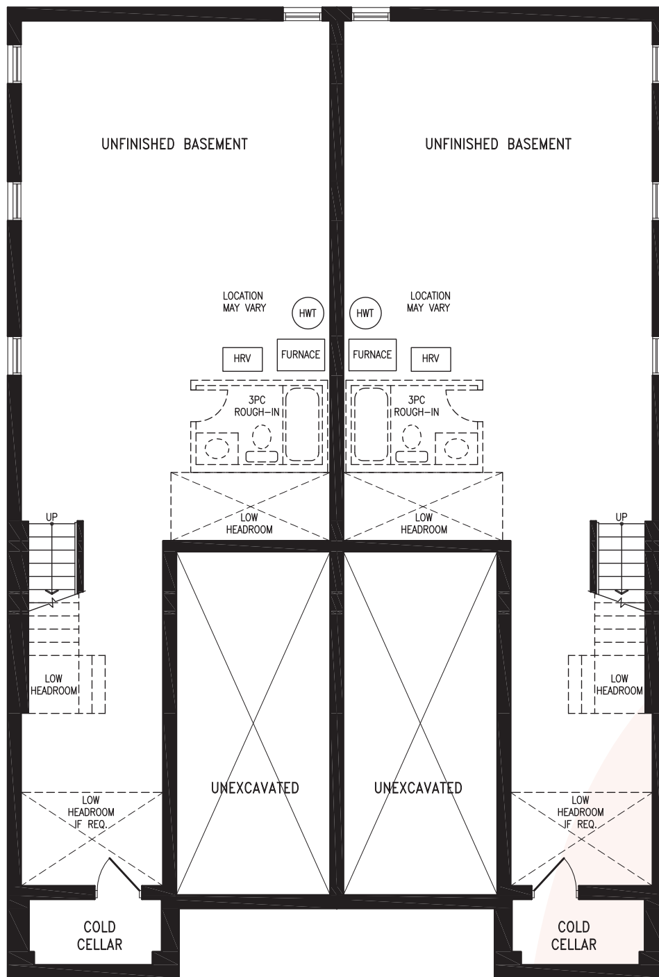
Elevation A1 BASEMENT
