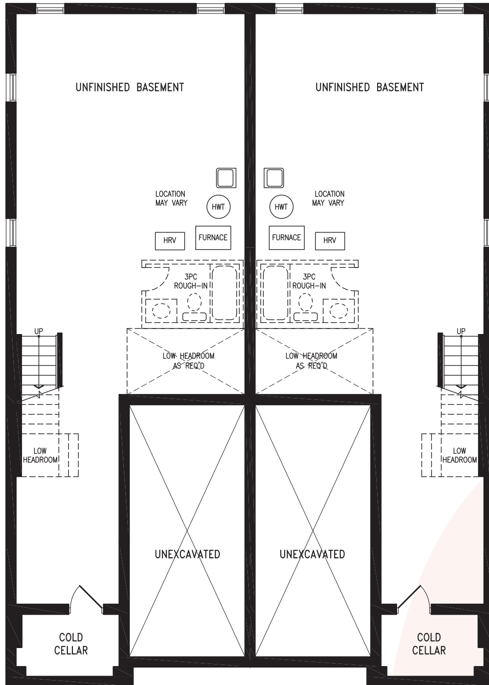
Elevation B1 BASEMENT
