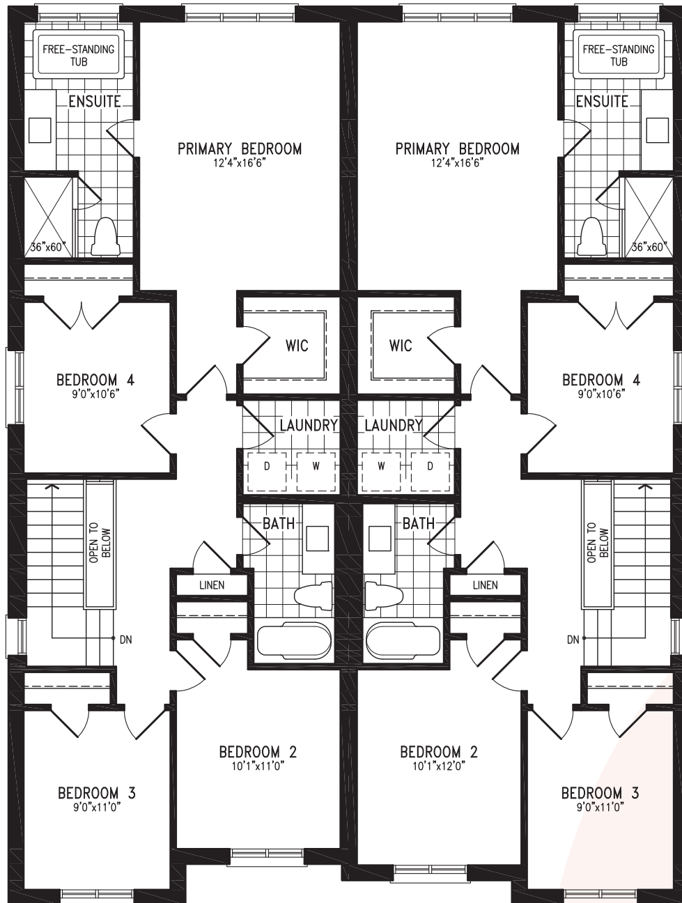
Elevation A1 SECOND FLOOR
