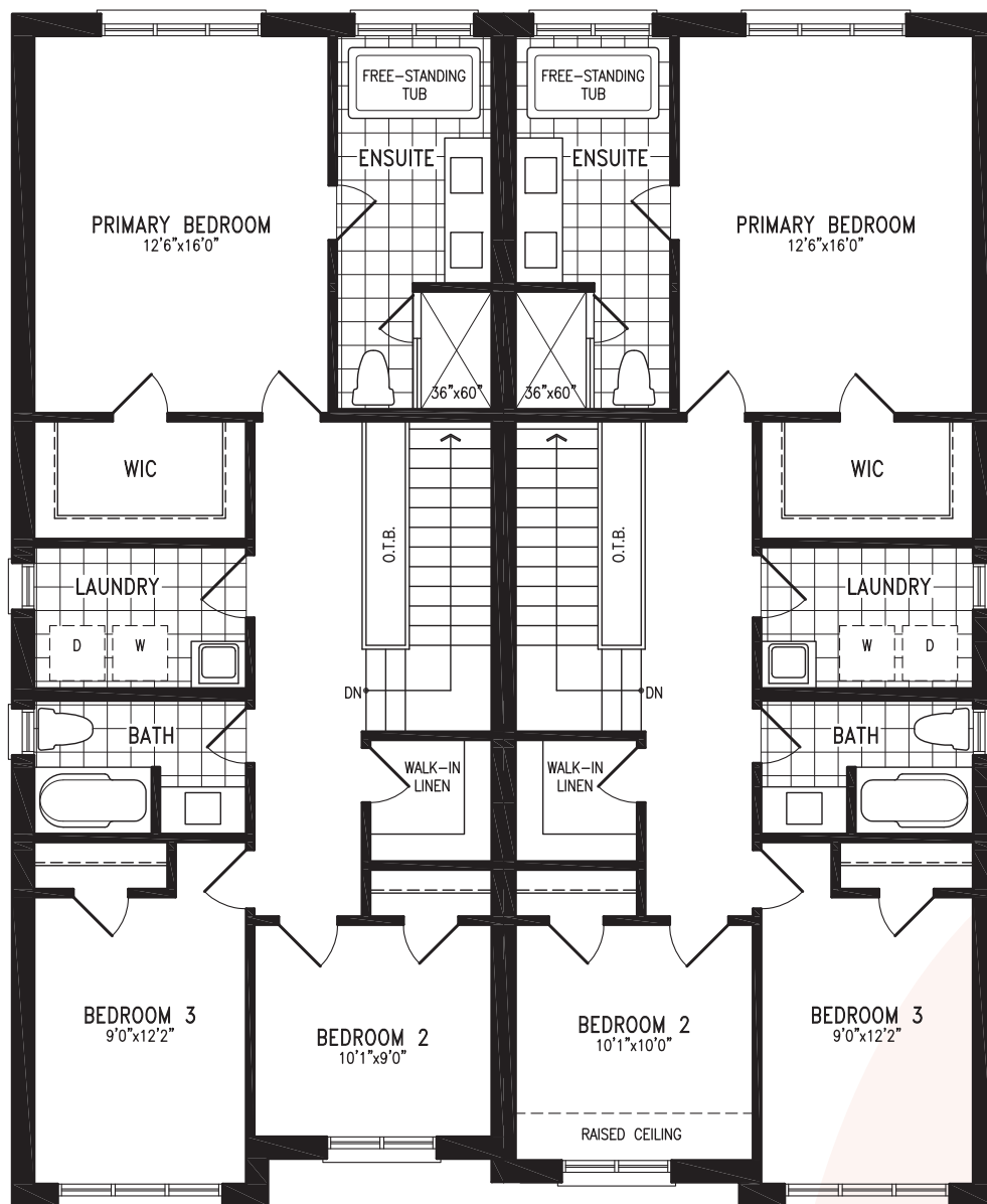
Elevation A1 SECOND FLOOR
