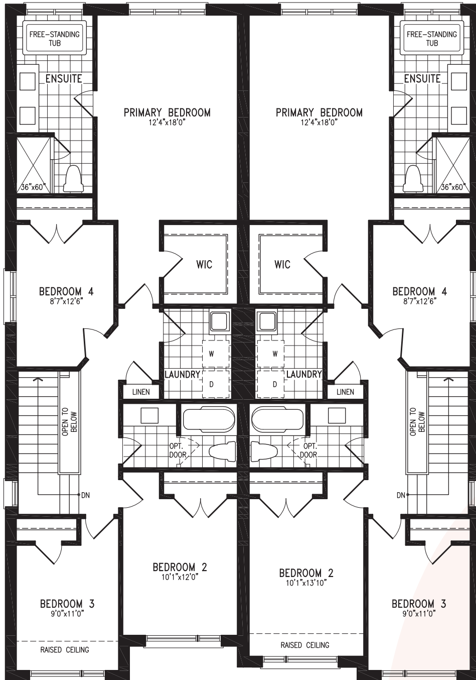
Elevation C1 SECOND FLOOR
